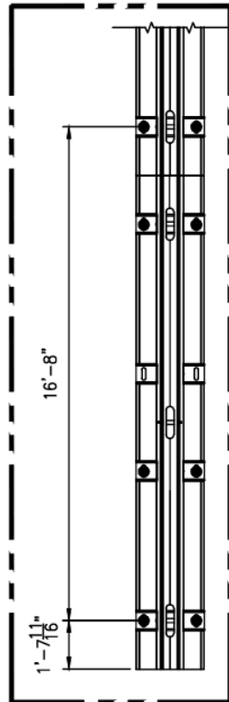
DETAIL 1 END ANCHORING WITH 7/8" Ø ANCHORS ON BRIDGE DECKS
