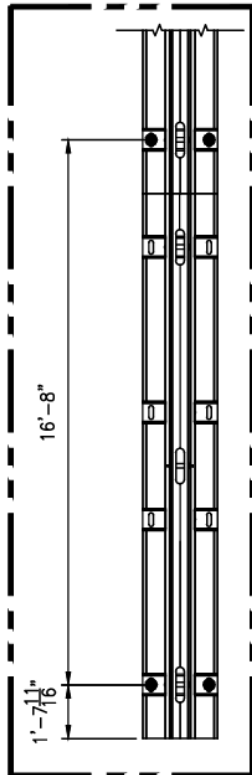
DETAIL 1 END ANCHORING WITH 1 1/2" Ø ANCHORS
