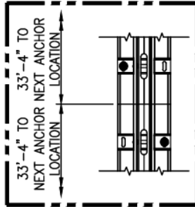
DETAIL 2 INTERMEDIATE ANCHORING WITH 1 1/2" Ø ANCHORS
