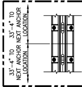
DETAIL 2 INTERMEDIATE ANCHORING WITH 7/8" Ø ANCHORS ON BRIDGE DECKS
