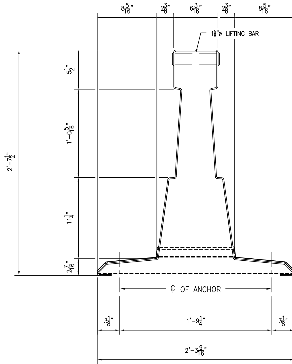
PROFILE AT ANCHOR POCKET
