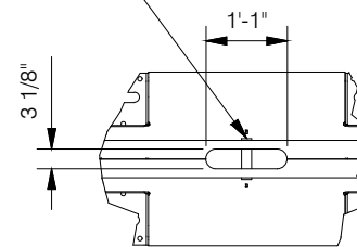
DETAIL A LIFT BAR DETAIL (TYP.)
