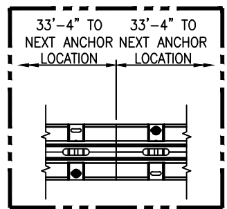
DETAIL 2 INTERMEDIATE ANCHORING WITH 1 1/4" ANCHORS
