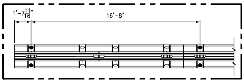
DETAIL 1 END ANCHORING WITH 1 1/4" ANCHORS
