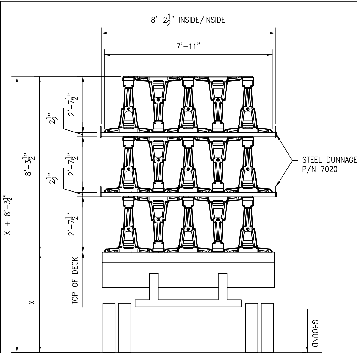
REAR VIEW
